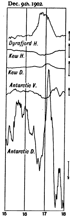
FIG. 33. ARCTIC-KEW-ANTARCTIC CURVES.
